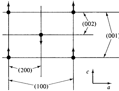
Fig. 5.15 Projection of the MnF_2 unit cell on a (010) face. Only the Mn ions are shown.
