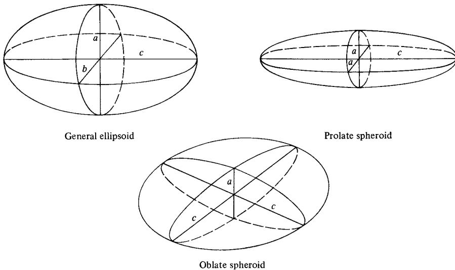
Fig. 2.27 Ellipsoids.
