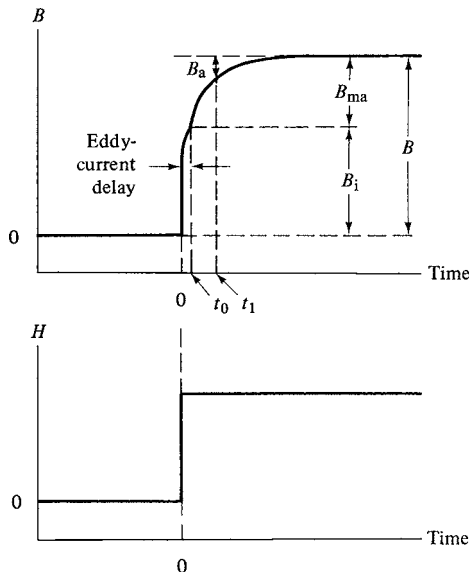
Fig. 12.13 Magnetic after-effect.
