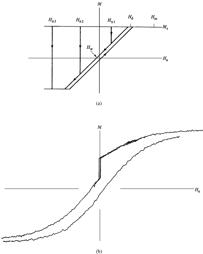
Fig. 11.16 Hysteresis loops of a single particle. (a) Theoretical. (b) Observed for a particle of \text{SmCo}_5 . [J. J. Becker, IEEE Trans. Mag. , 5 (1969) p. 211.]
