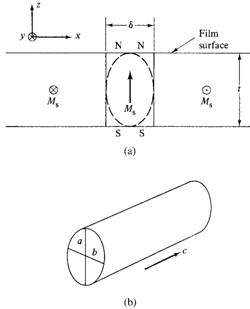
Fig. 11.30 (a) Cross section of 180^\circ Bloch wall in thin film. (b) Elliptic cylinder.
