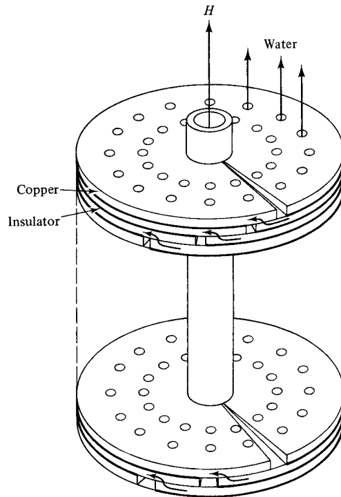
Fig. 2.5 Sketch of a Bitter magnet solenoid. Arrows indicate the current path from one disk to another.
