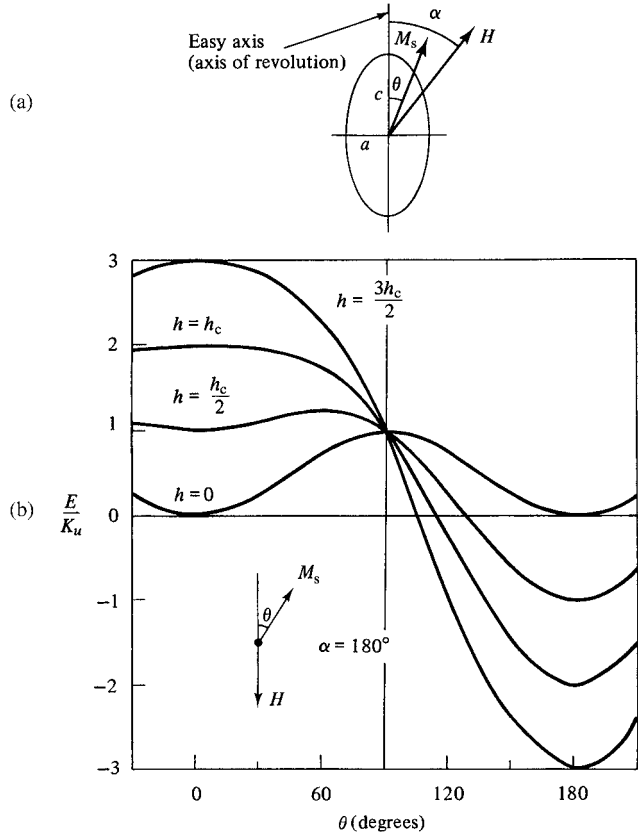
Fig. 9.35 Rotation of magnetization by a field applied to a single-domain ellipsoid; h is a reduced field H/H_K (see text).
