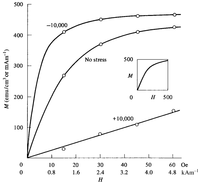
Fig. 8.16 Effect of applied tensile (+) and compressive (−) stress on the magnetization curve of polycrystalline nickel; 10,000 \text{ lb/in}^2 \approx 69 \text{ MPa} . [D. K. Bagchi, unpublished.]
