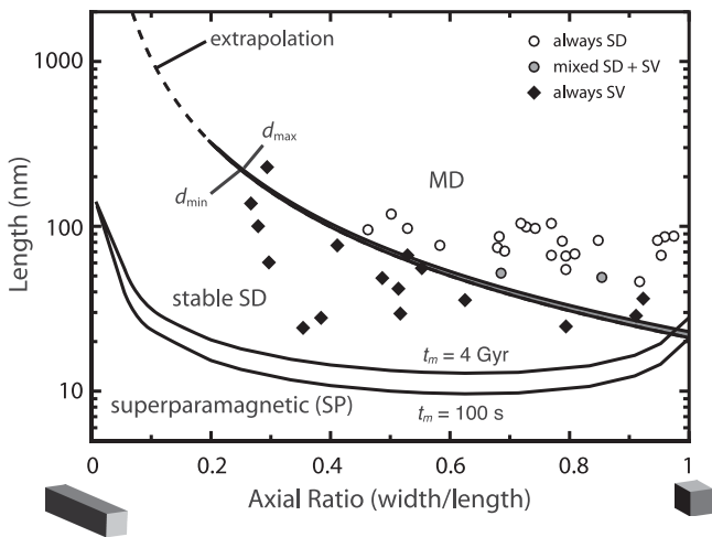
Figure 5. Stable SD grain size ranges for individual particles of metallic iron. Grain elongation is in the (100) direction. The grey area between d_{\max} and d_{\min} indicates the range where both SD and SV (MD) states are possible. For the SP/SD transition lines are for t_m = 100 s and 4 Gyr at 300 K. Published domain-state observational data for 40 Fe–Ni particles in synthetic ‘dusty olivines’ are also plotted (Lappe et al. 2011). Lappe et al. (2011) examined each particle more than once, and determined whether they were always SD, always SV (MD) or displayed mixed states. Increasing levels of Ni, will increase the SD to MD transition size.
